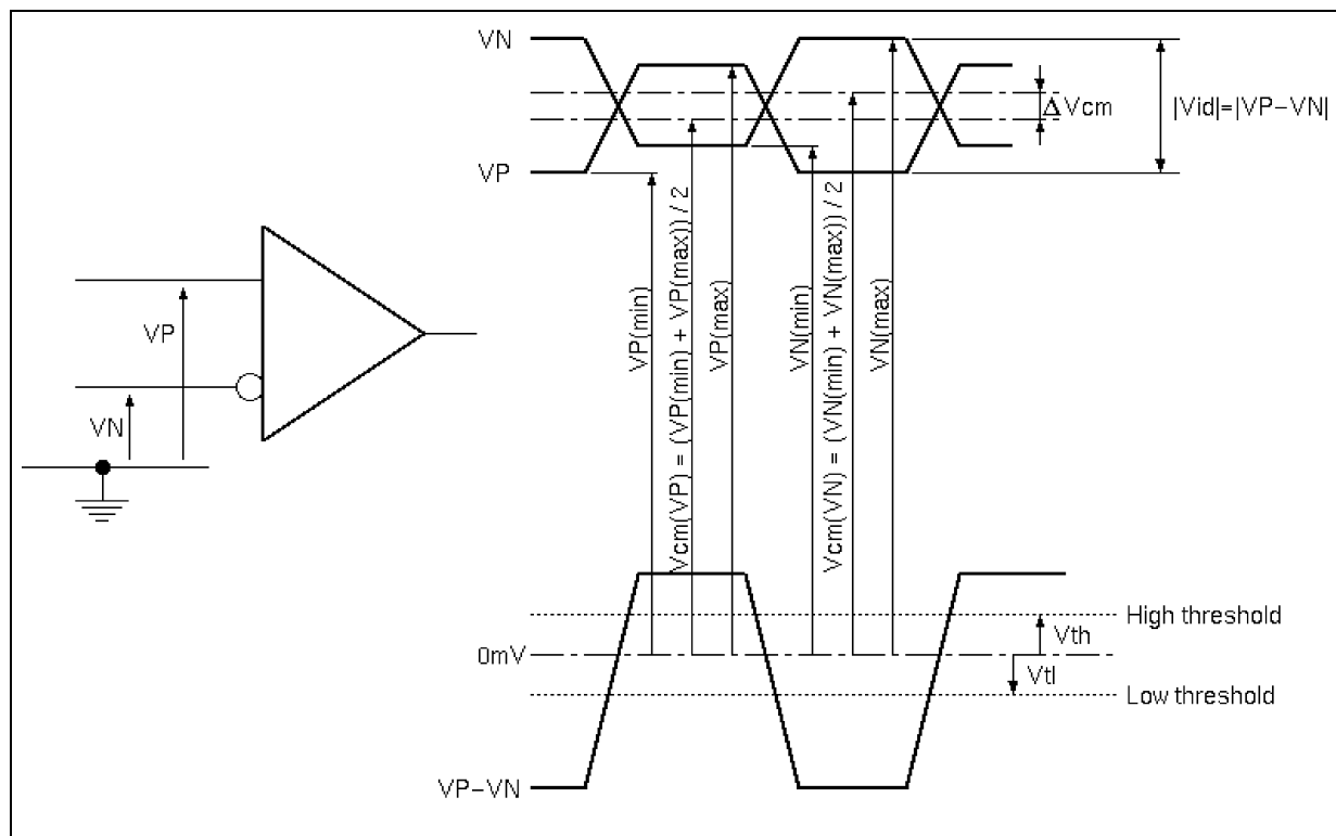
Voltage Definitions
